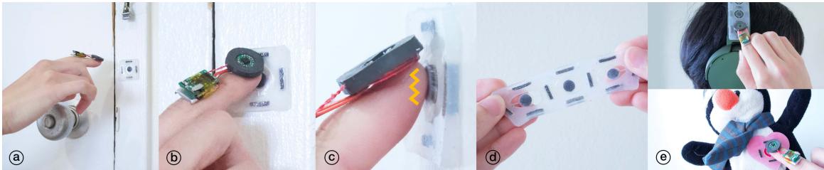
Figure 1: (a) We demonstrate a new type of haptic actuator, which we call MagnetIO, that is comprised of two parts: any number of soft interactive patches that can be applied anywhere and one battery-powered voice-coil worn on the user's fingernail. (b) When the fingernail-worn device contacts any of the interactive patches it detects its magnetic signature and (c) makes the patch vibrate . (d) To allow these otherwise passive patches to vibrate, we make them from silicone with regions doped with neodymium powder, resulting in soft and stretchable magnets. (e) This novel decoupling of traditional vibration motors allows users to add interactive patches to their surroundings by attaching them to walls, objects or even other devices or appliances without instrumenting the object with electronics.
