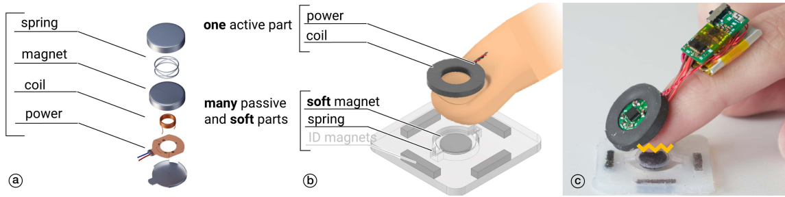
Figure 2: (a) Our device is built from the same principle as traditional linear resonant actuators (LRA). (b-c) However, our device decouples these components into two parts: one active element containing the coil, worn on the user’s fingernail; and, many passive elements, which are comprised of silicone with regions doped with neodymium powder which together realize a spring & magnet.
